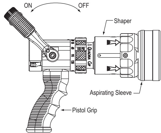
QUADRACUP & NAVCUP EXTENDED POSITION Figure 3.1F
