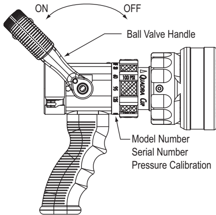
QUADRACUP & NAVCUP RETRACTED POSITION Figure 3.1E
