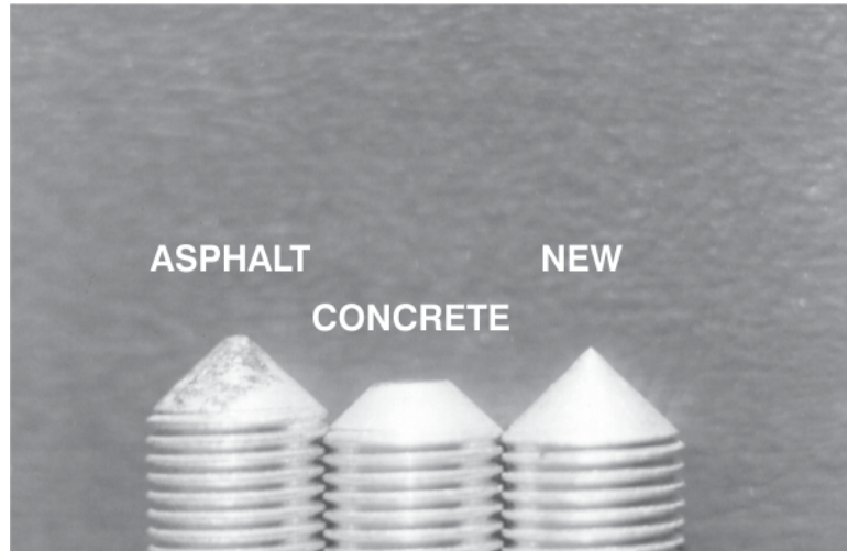
Results of ELKHART STINGER® being dragged 30 feet.
