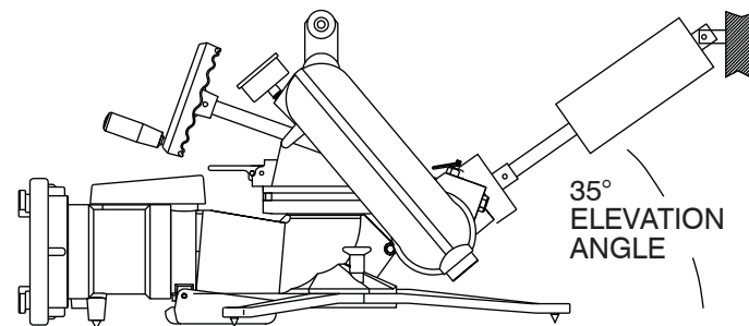
FIGURE 1 SLIDING TEST
