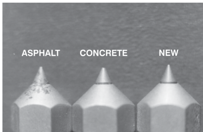
Results of TASK FORCE TIPS CROSSFIRE® being dragged 30 feet.
