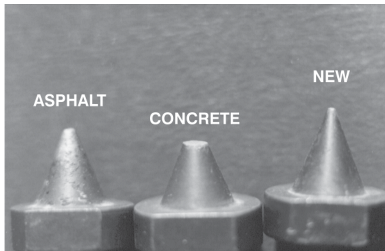
Results of AKRON APOLLO® being dragged 30 feet.
