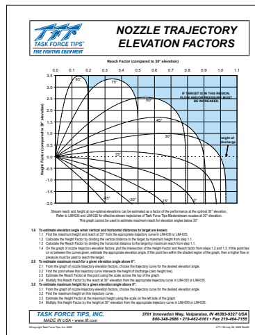
LTT-135 Nozzle Trajectory Elevation Factors
