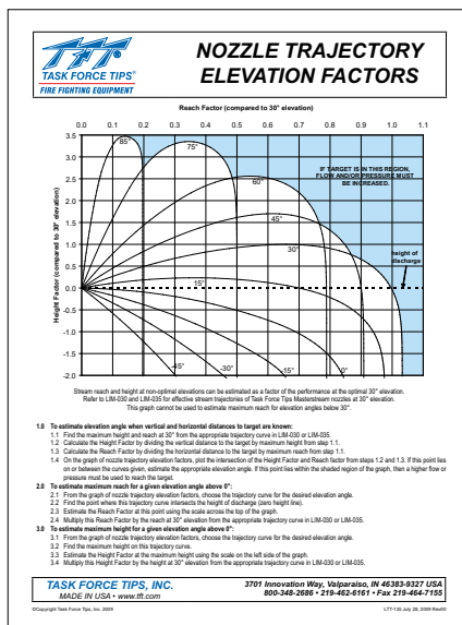
LTT-135 Nozzle Trajectory Elevation Factors
