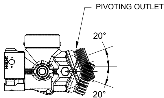
2.5" IN-LINE PIVOTING
