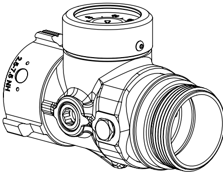
2.5" IN-LINE PIVOTING
