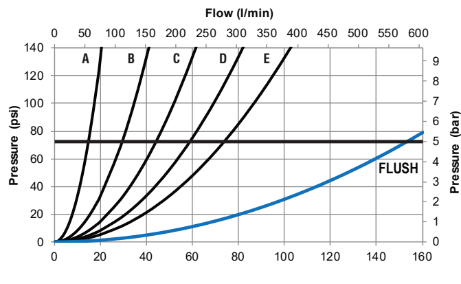
Figure 4.2D 1.0" / 25 mm G-Force 75 psi / 5 bar Fixed and Selectable Nozzles
