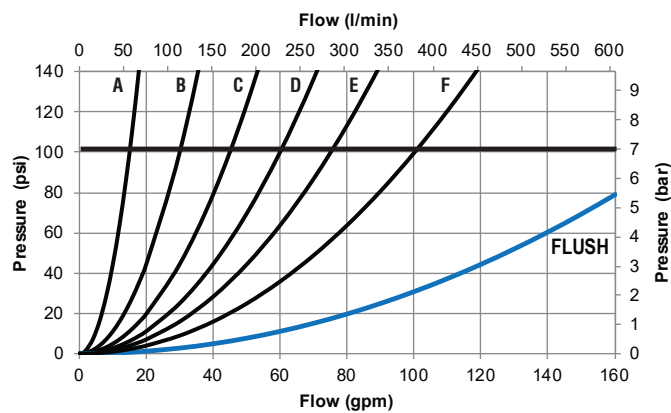
Figure 4.2C 1.0" / 25 mm G-Force 100 psi / 7 bar Fixed and Selectable Nozzles
