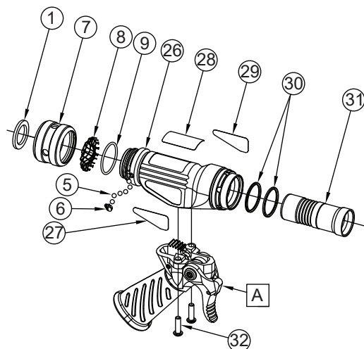
E - TN910GD / TN910GDHP SUBASSEMBLY
