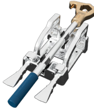
3 WRENCH BRACKET SET A3845
