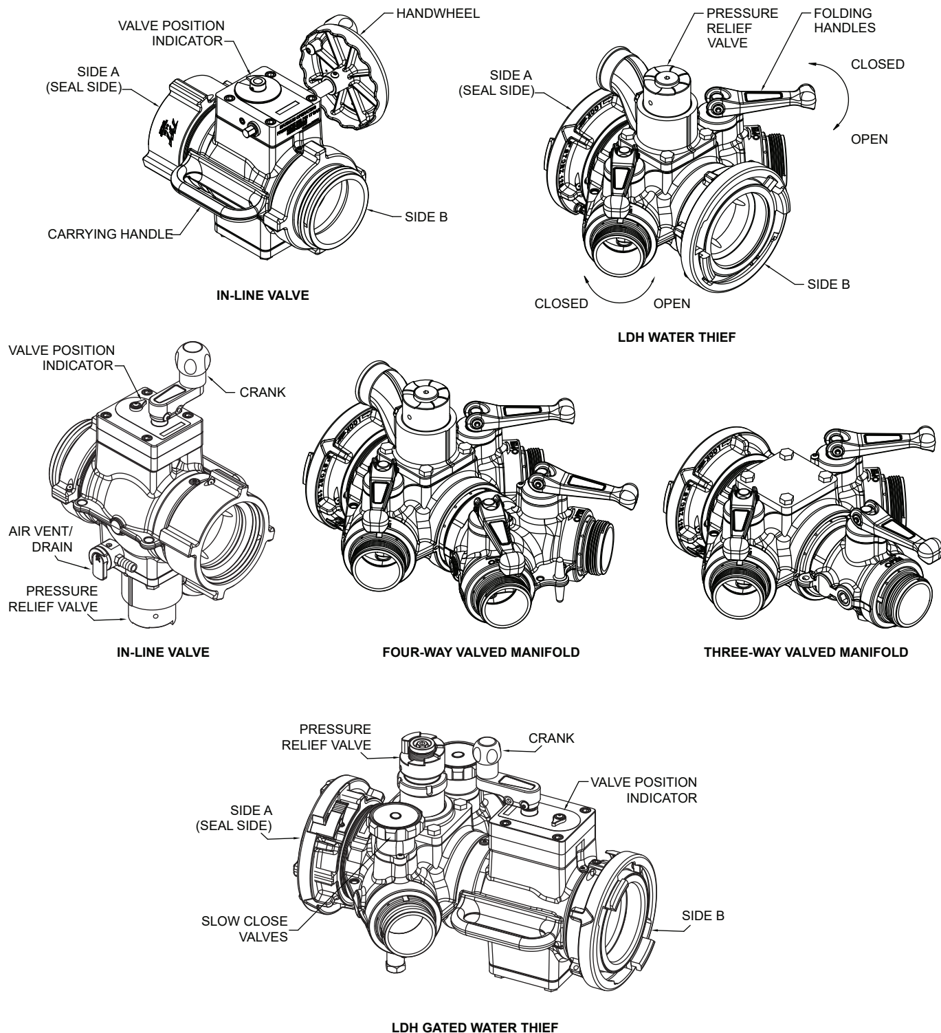
Figure 3.1 Parts Identification
