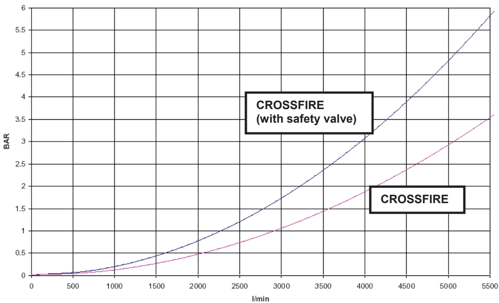
Figure B.1- Pressure loss chart
